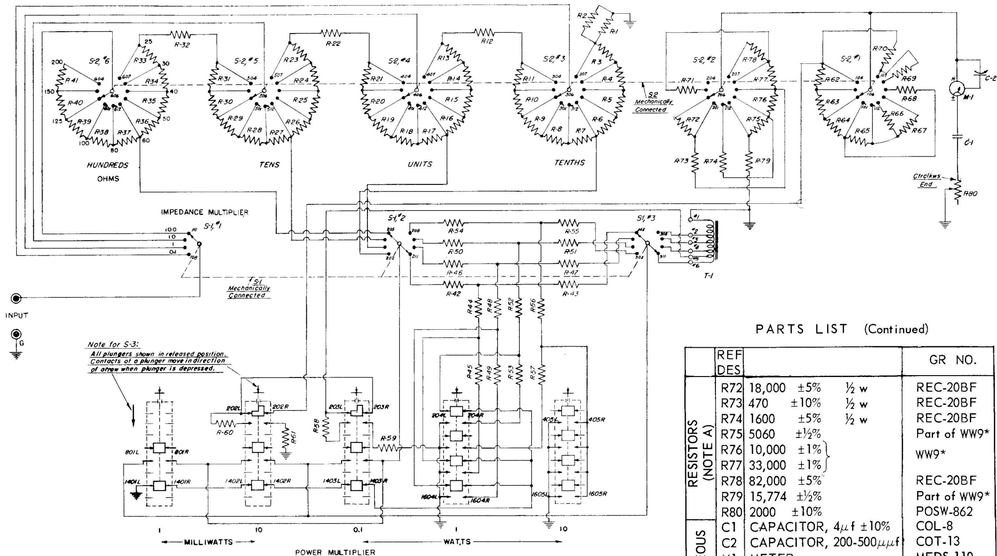
Figure 4. Schematic Diagram
